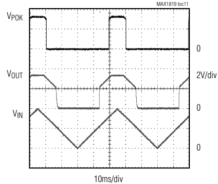
POWER-ON RESET
