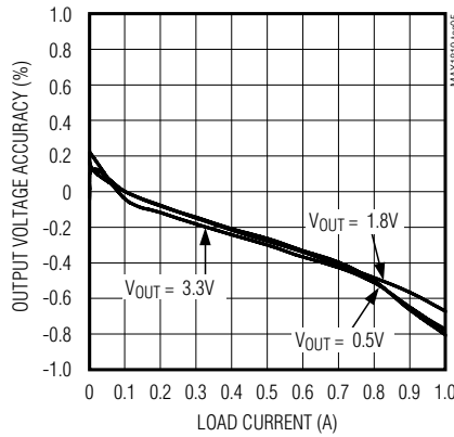
OUTPUT VOLTAGE ACCURACY vs. LOAD CURRENT
