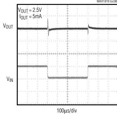
LINE TRANSIENT
