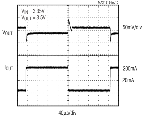
LOAD TRANSIENT RESPONSE NEAR DROPOUT
